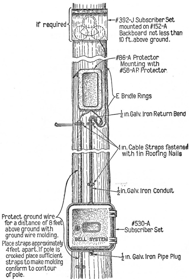
Figure 2. Pole Installation
